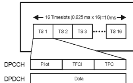
Frame structure
